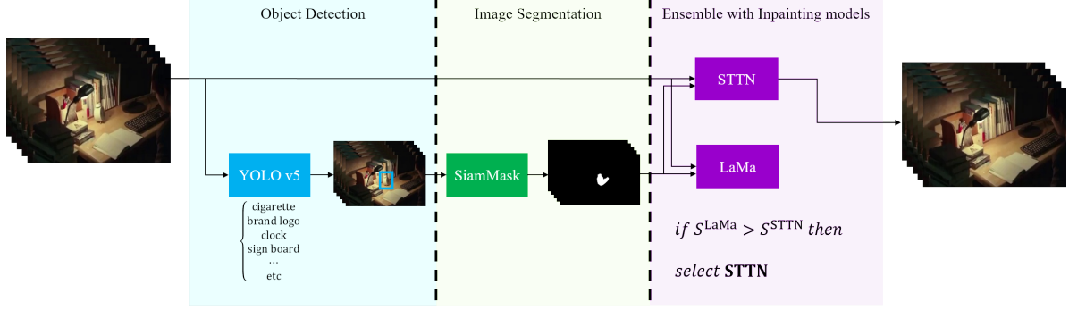
Figure 3. The architecture of our model. YOLOv5 takes frames of an original video as input, and feeds their results to SiamMask to output the mask images. Then, two different inpainting modules take original frames and their mask images as input and produce respective results. The best of these is determined by the final result using proposed NR-VQA.
